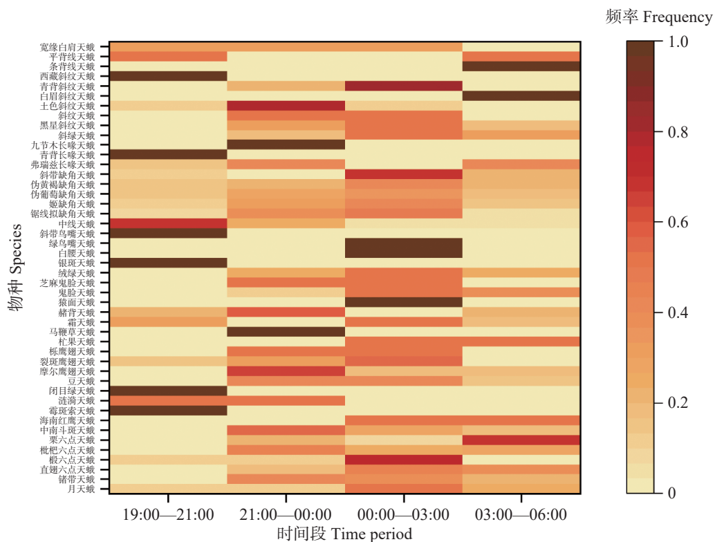
图 5 黎母山景区天蛾科昆虫不同时间段的上灯频率 Fig. 5 Light-attraction frequency of Sphingidae at different time periods in Limu Mountain scenic area
