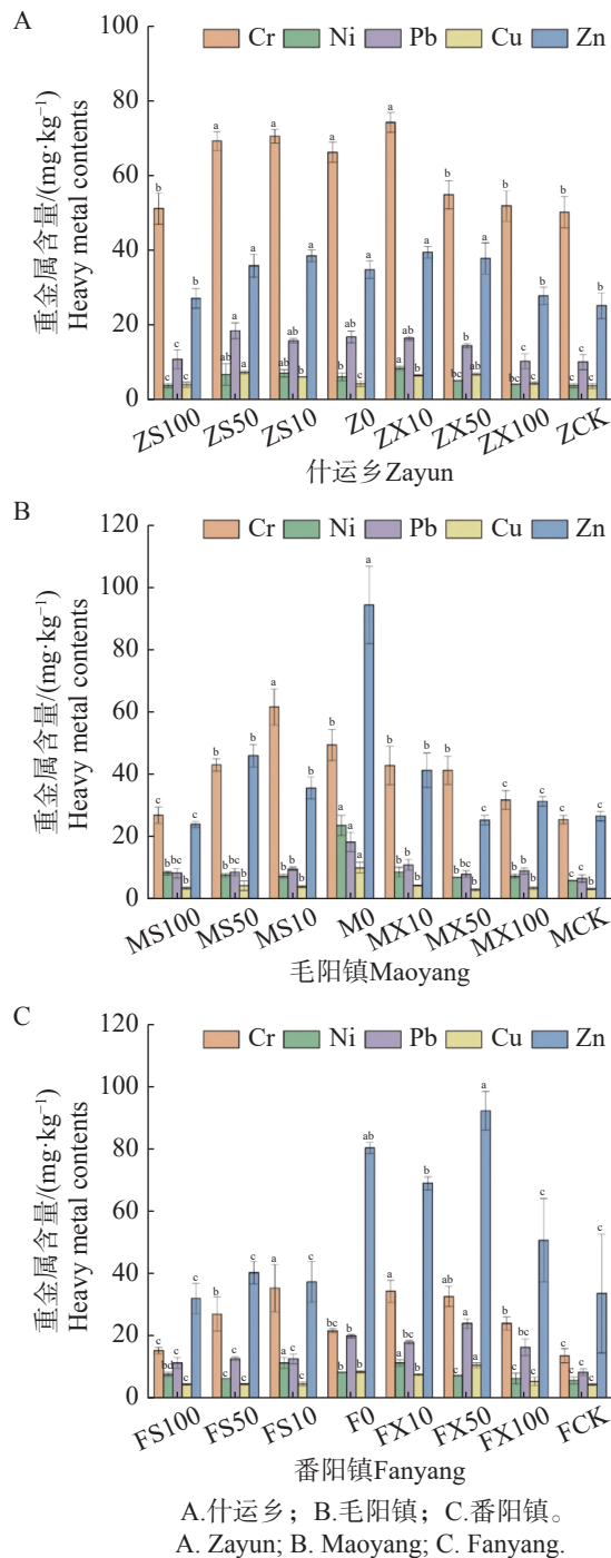
Fig. 1 Spatial distribution pattern of soil heavy metals
