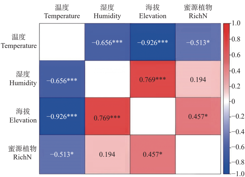
图 2 影响因子间相关性分析结果 Fig. 2 Results of mantel correlation tests between influencing factor
